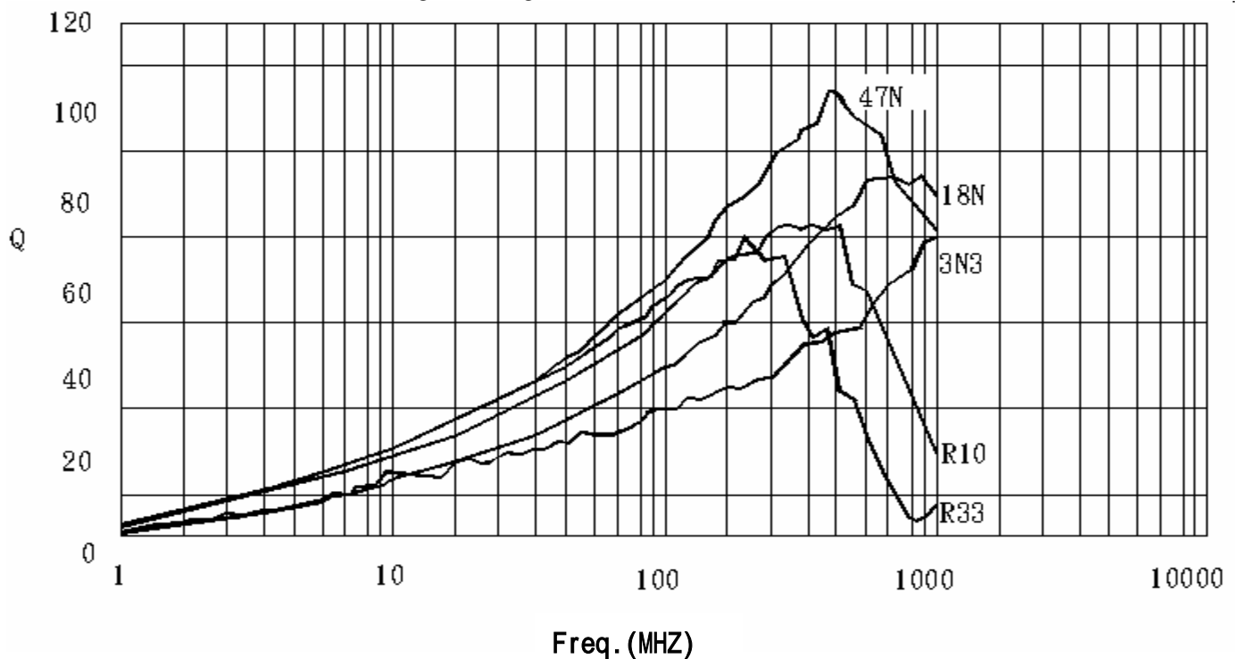
Q vs. FREQUENCY CHARACTERISTICS
