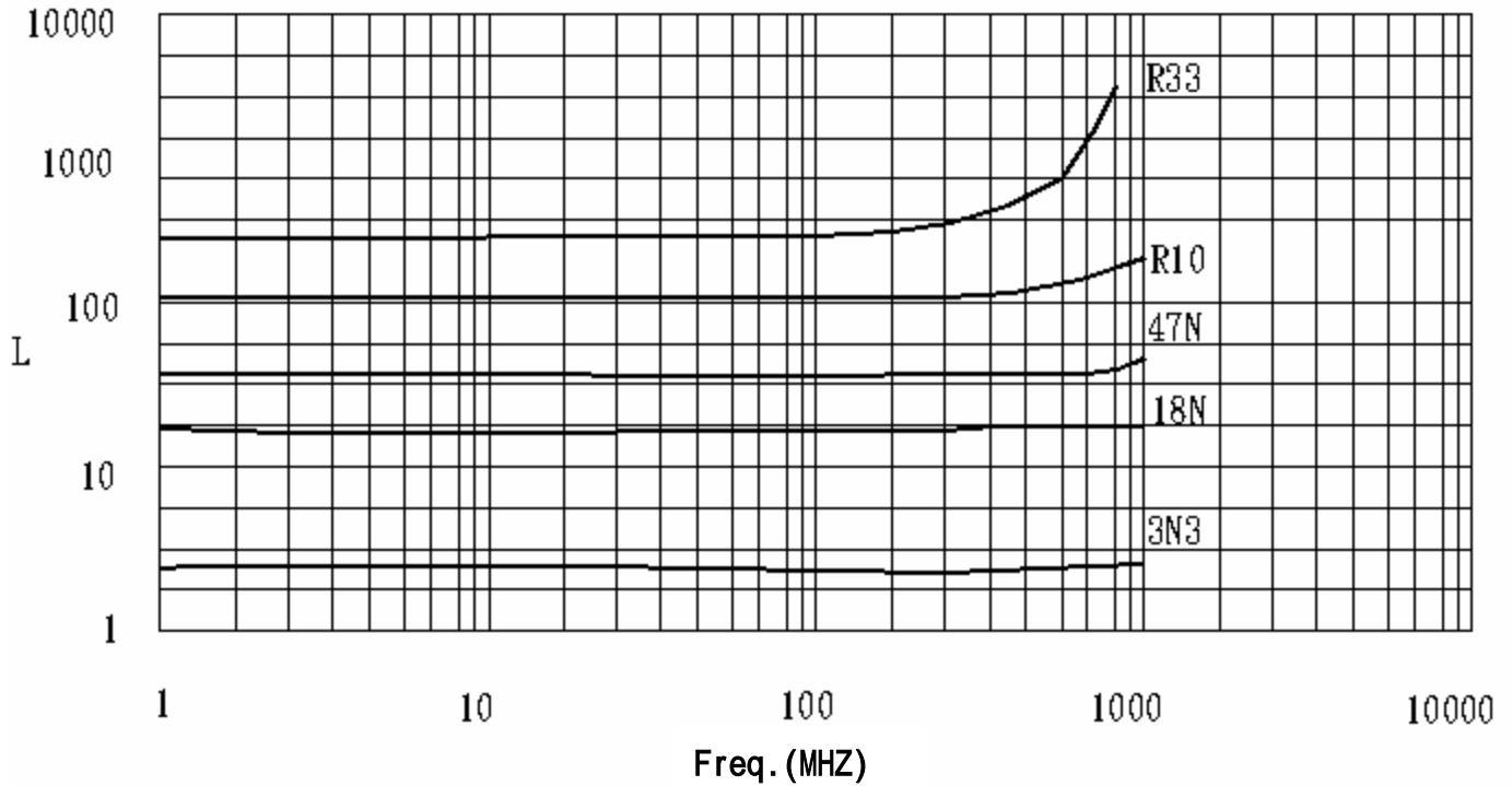
INDUCTANCE vs. FREQUENCY CHARACTERISTICS
